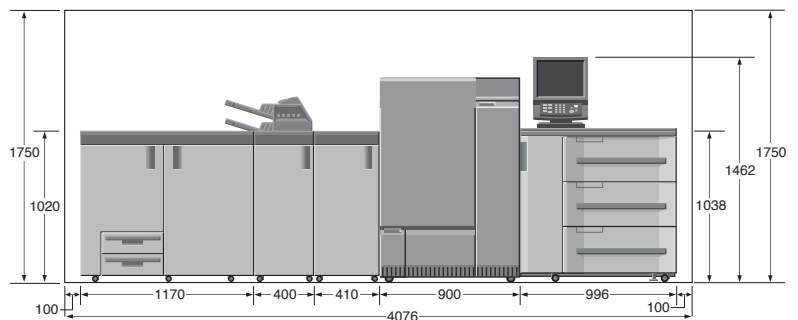
Front View bizhub PRESS C1100 / C1085 + SD-506 + FD-503 + RU-511 + PF-707
