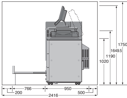
Side View bizhub PRESS C1100 / C1085 + SD-506 + RU-511 + WT-512 + PF-708
