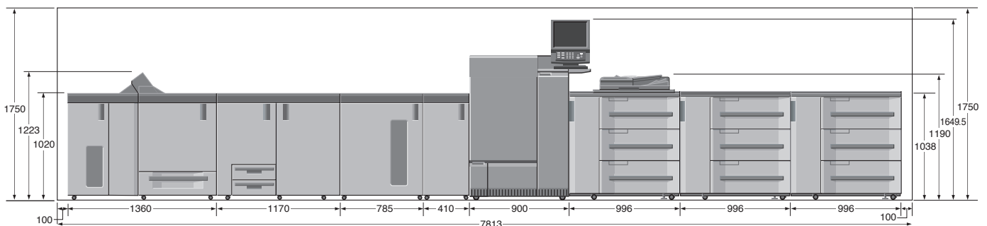
Front View bizhub PRESS C1100 / C1085 + PB-503 + SD-506 + LS-506 + RU-511 + WT-512 + PF-708 + PF-707 + PF-707
