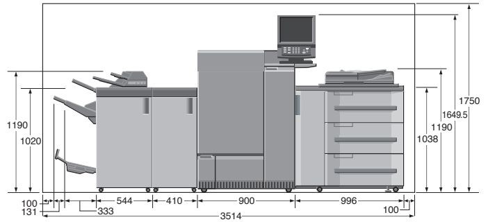
Front View bizhub PRESS C1100 / C1085 + FS-532 (PI-502/MK-732/PK-522/SD-510) + RU-511 + WT-512 + PF-708
