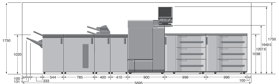
Front View bizhub PRESS C1100 / C1085 + FS-532 + LS-506 + FD-503 + RU-511 + WT-512 + PF-707 + PF-707
